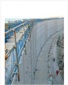
The tsunami barrier being built at Chubu Electric Power Co.'s Hamaoka Nuclear Power Plant is pictured in Omaezaki, Shizuoka Prefecture, on Dec. 27. (Mainichi)
