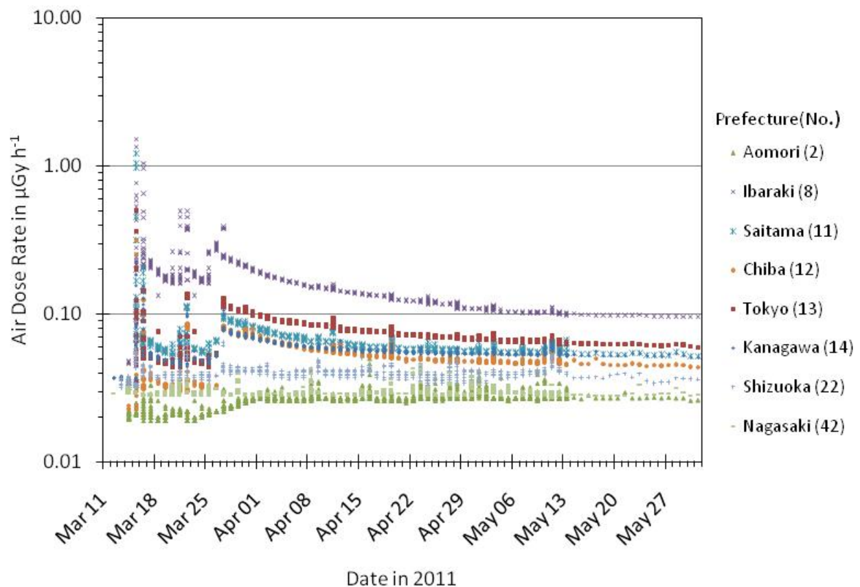
Figure 29. External radiation dose rates from MEXT data in prefectures with DOD-affiliated individuals
